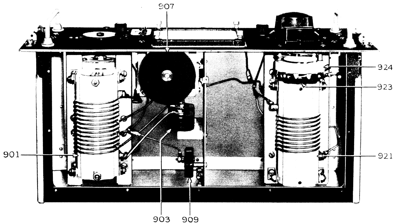
FIGURE 38. TRANSMITTER TUNING UNIT TU-9-B, BOTTOM VIEW, COVER REMOVED
